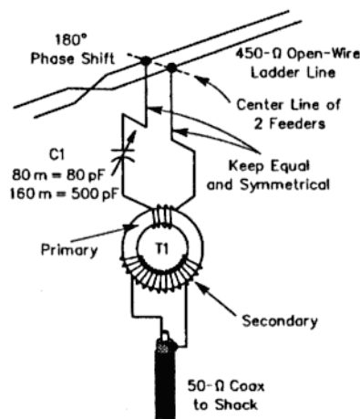
Figure 2-Details of the matching network for 80 and 160-meter single-band operation when using 450-a open-wire ladder line. This network is included inside the junction box (see Figure 1) of each 80 and 160-meter antenna.
