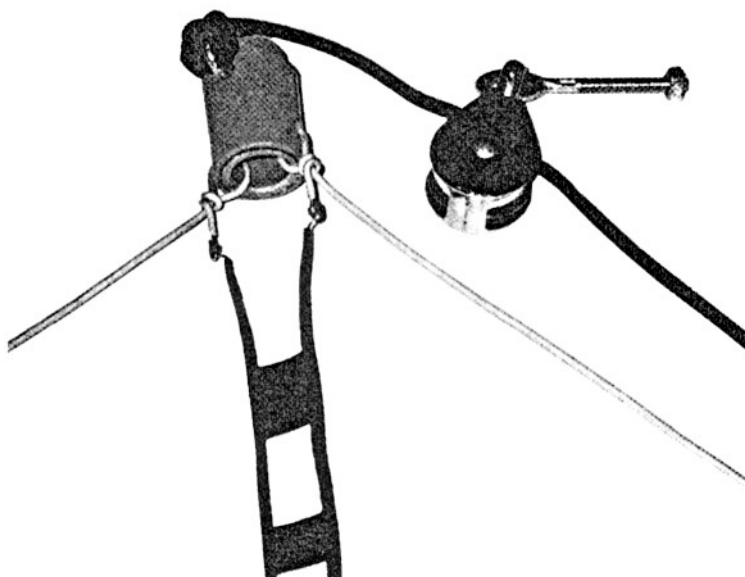
Figure 5-Attachment of the 450 \Omega line to the antenna arms and homemade PVC support insulator.
