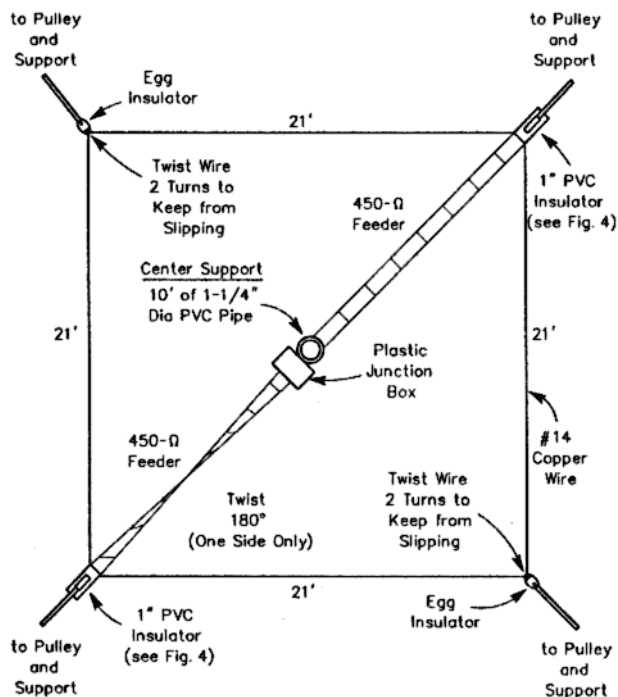
Figure 1-Looking down on the K6STI square - an 80 and 160 meter antenna that reduces interference from powerline noise. At W6KUT's location the antenna is installed at a height of 10 feet. A 10 foot long 1 1/4" diameter PVC pipe acts as a center support.
