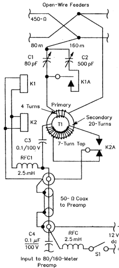
Figure 3-Matching network for a duoband (80 and 160-meter) K6STI Square. Relays, powered through the coaxial-cable feed line, provide the required LC switching.
